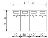
EXCEPTION DIMENSIONS FOR LOTS 1-30
